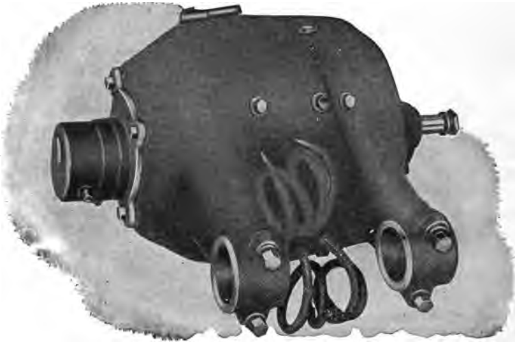
FIG. 293.—General Electric Motor, Designed for Heavy Vehicle Use, with single or double reduction. Capacity, 30 amperes at 85 volts; 800 R. P. M. at full load.
